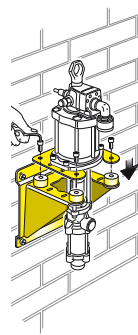
Art. 10/18 Wall bracket in painted steel with dampers for wall-mounting of divorced industrial pumps, with suction tube Ø 100 mm, series 900 and 1200
