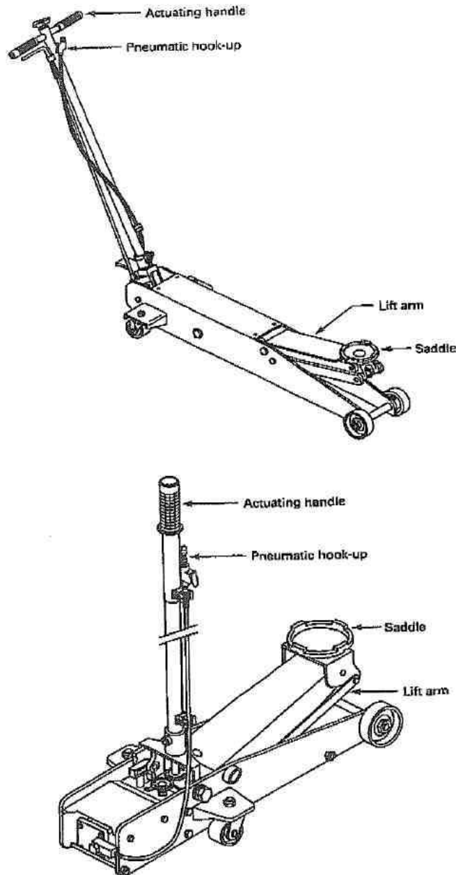
Fig. 10-2 Typical Pneumatic/Hydraulic Service Jacks
